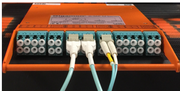
Figure 11 LC Connectors connected to TAP
